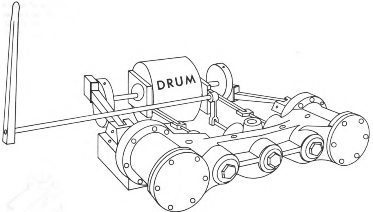
Figure 8-10. Two-cylinder steam feed works.
